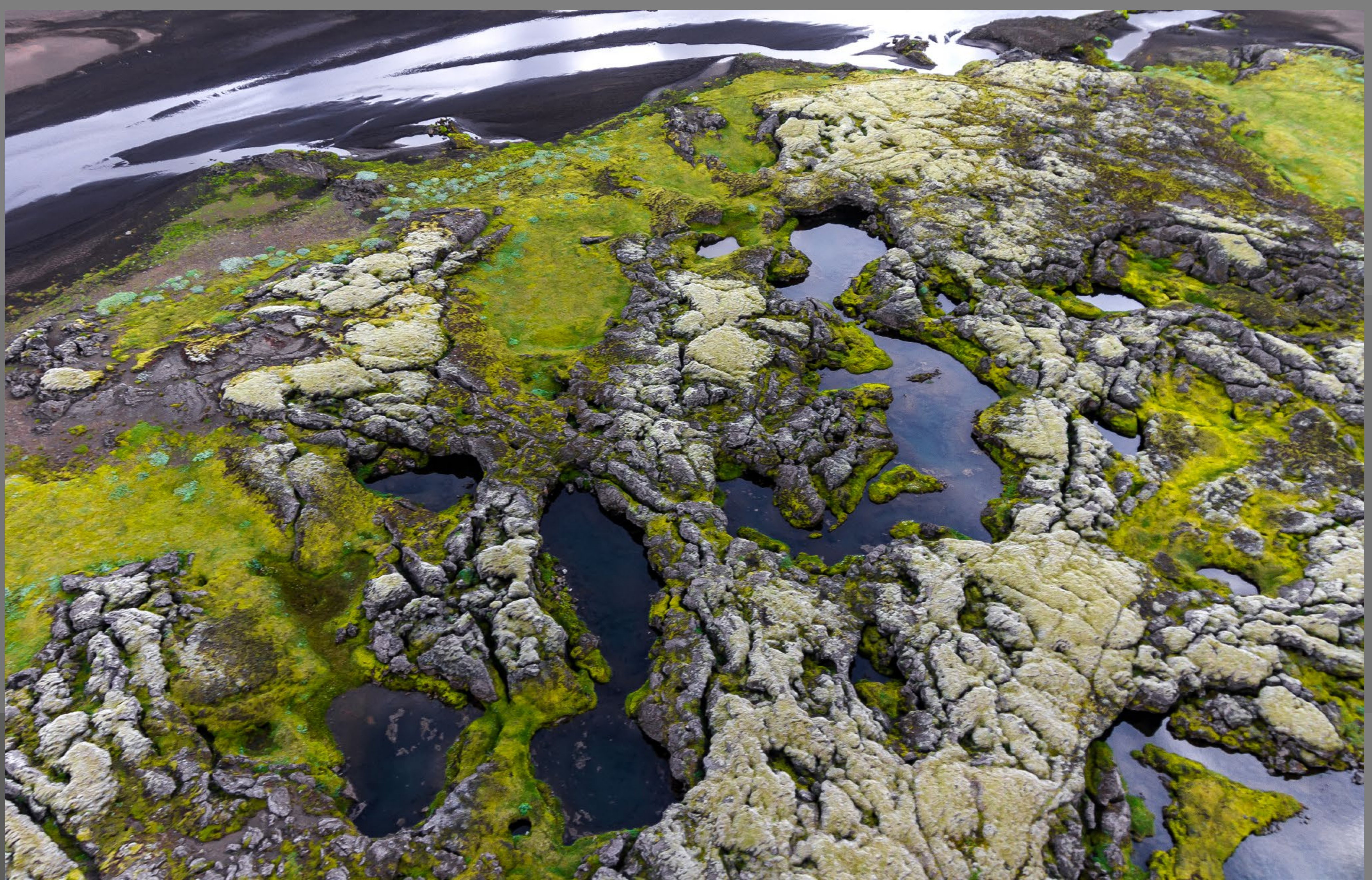
Patterns in Tjarnarhraun Lava
