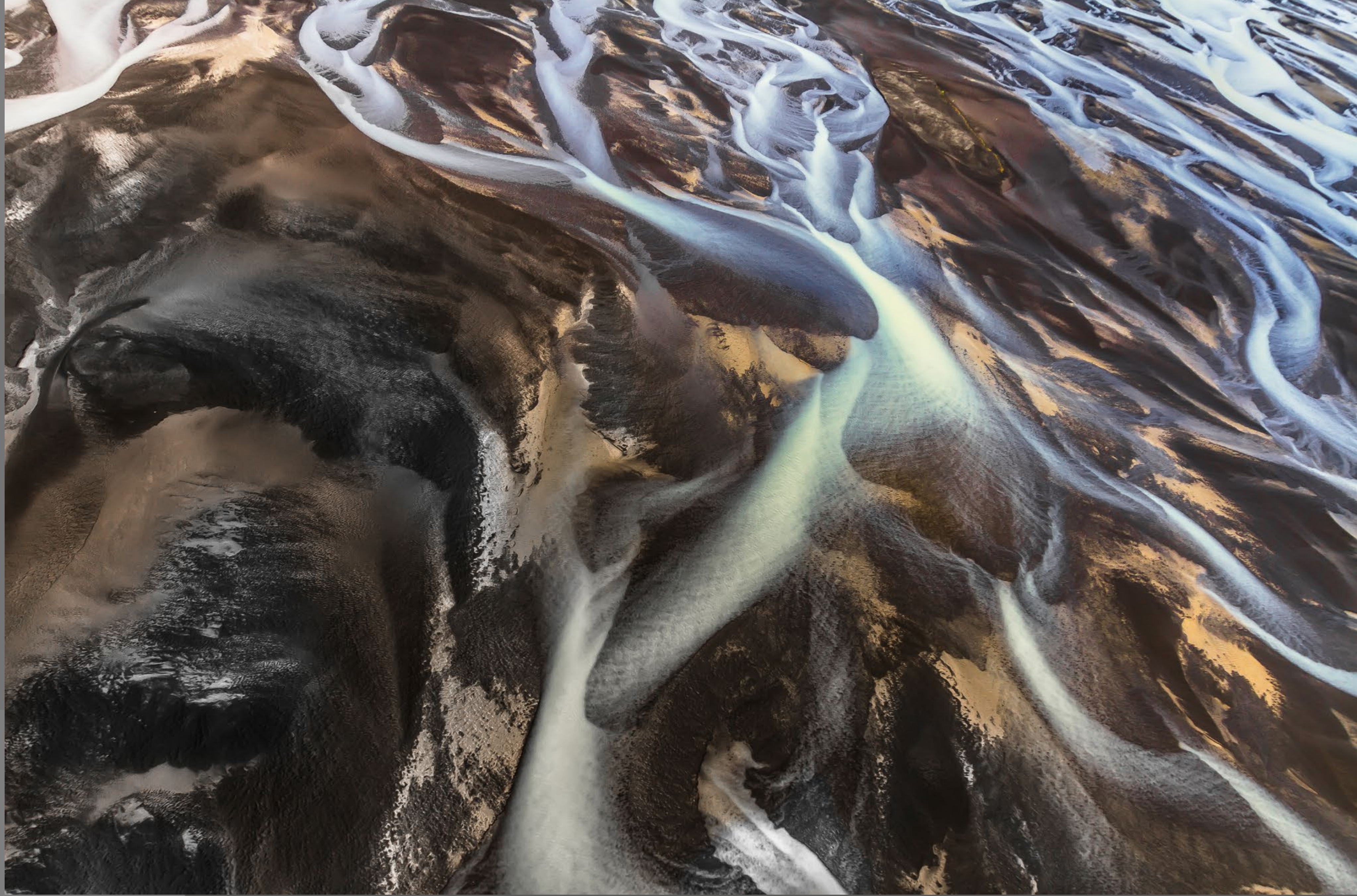
River Patterns
